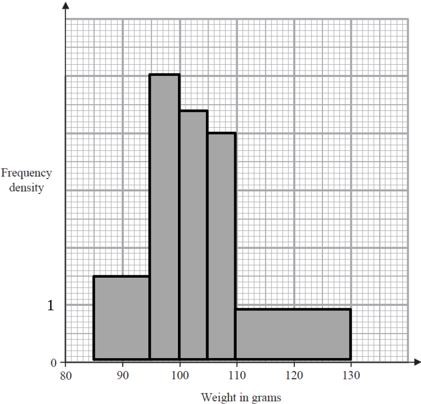
Commonly seen correct Histograms
