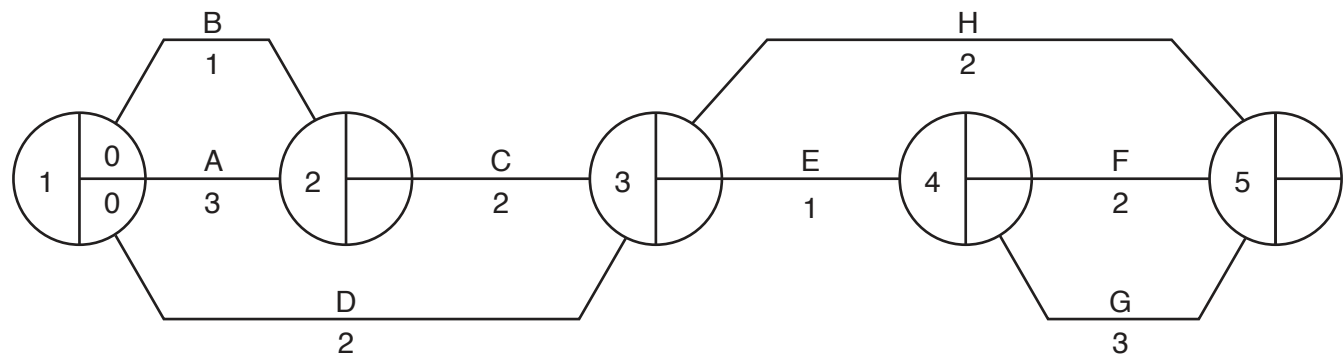
Appendix A: Network for assembling a kit house
