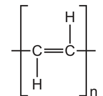
poly(acetylene)
