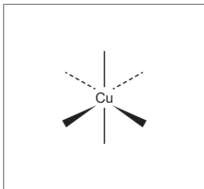
isomer 1
