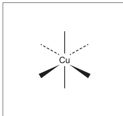
isomer 2
