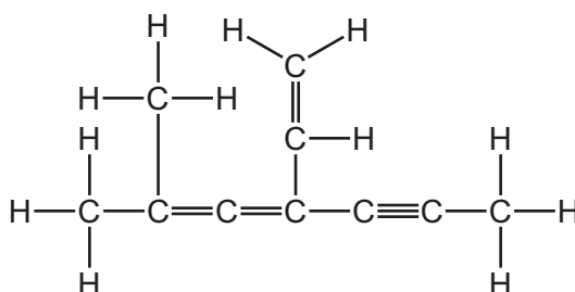
molecule Q
