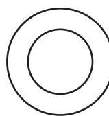
fluoride ion
