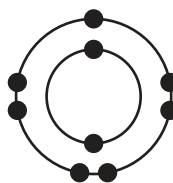
fluorine atom
