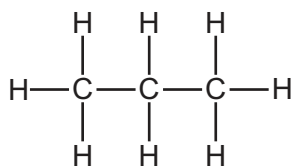
compound F
